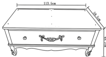
Base unit
